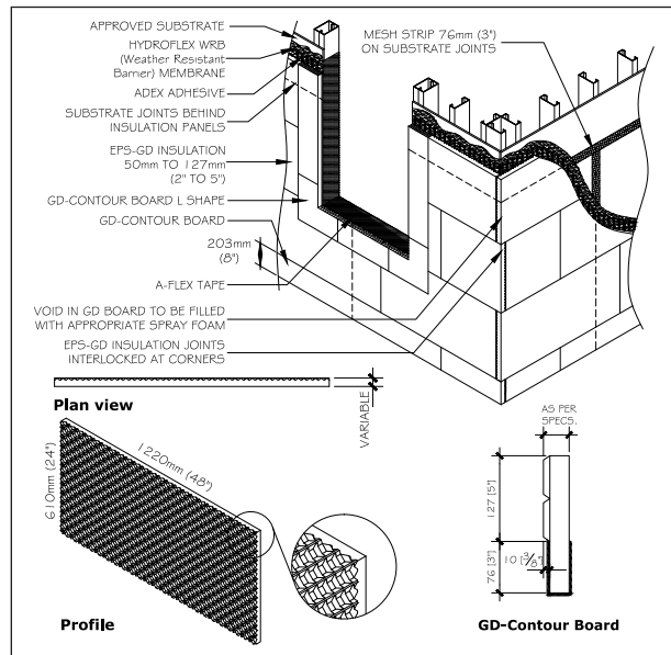
INSULATION INSTALLATION - METHOD 2
