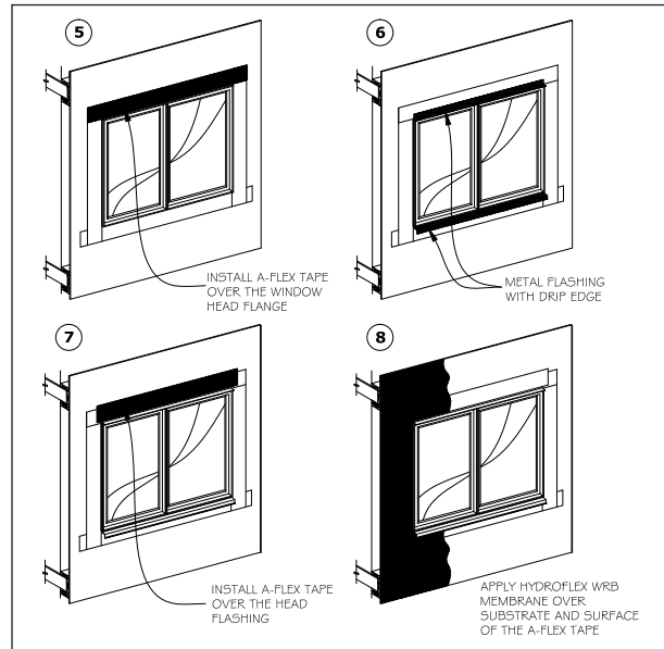
WINDOW TREATMENT - PART 2
