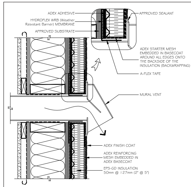
WALL PENETRATIONS
