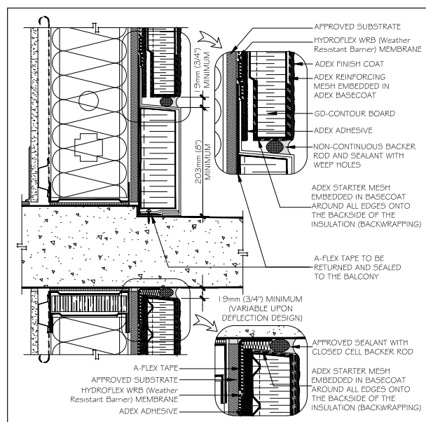
BALCONY JUNCTION
