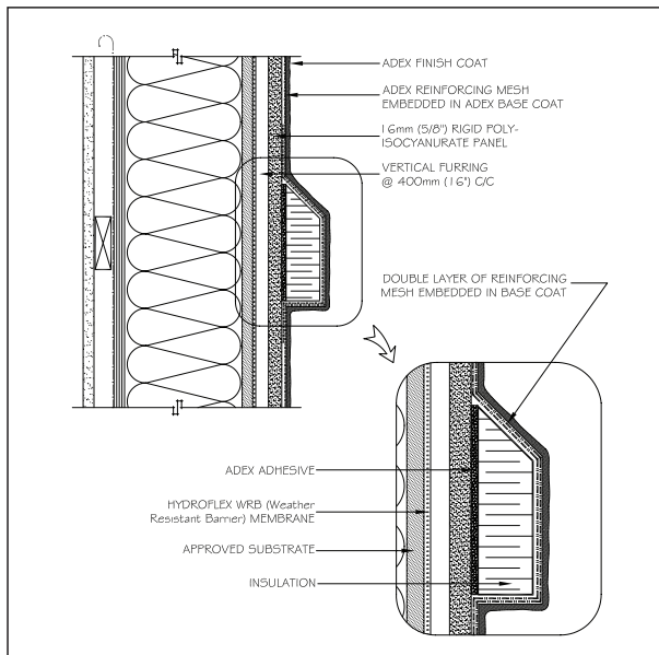
DECORATIVE BAND
