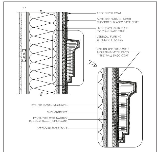
PRE-BASED MOULDING
